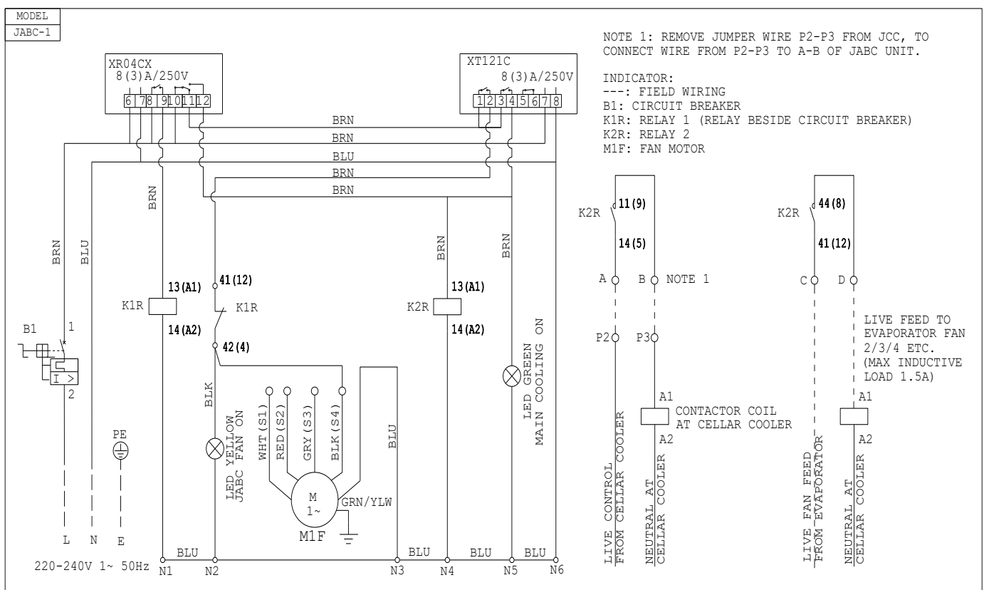
Figure 8: Wiring Diagram
