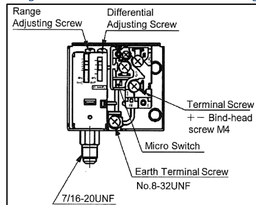
Figure 6: Low Pressure Switch Setting
