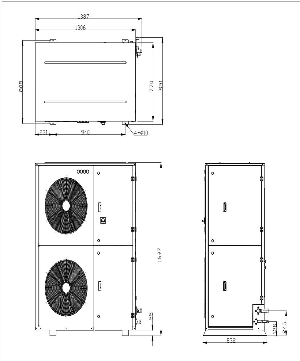
Figure 20: Outline Drawing JEHSDT-1201-B5-M-3
