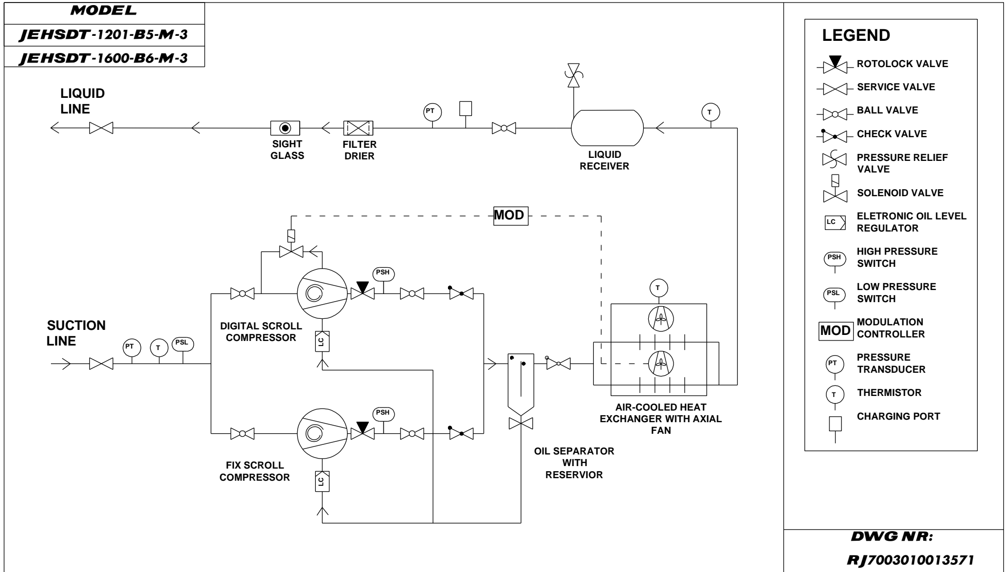
Figure 23: P&I Diagram
