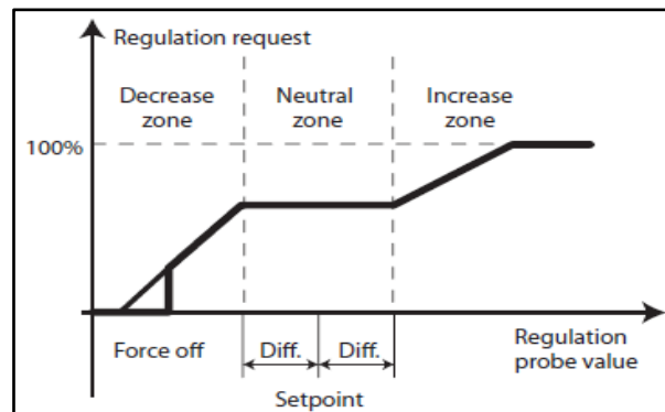
Figure 14: Regulation Request Versus Setpoint
