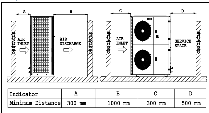
Figure 9: Installation Clearance
