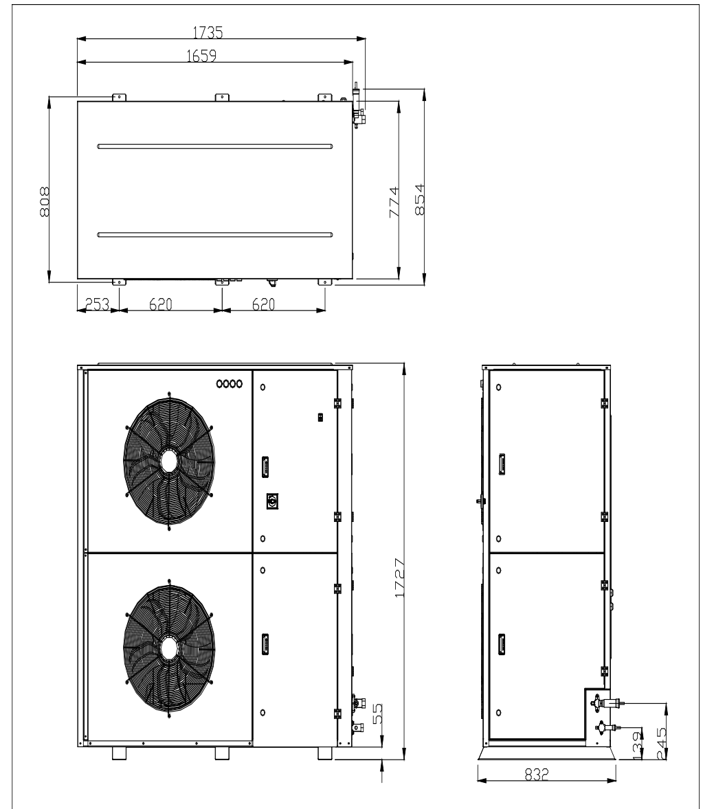
Figure 21: Outline Drawing JEHSDT-1600-B6-M-3
