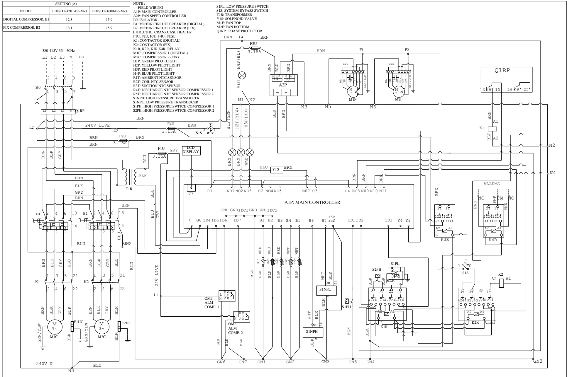
Figure 22: Wiring Diagram
