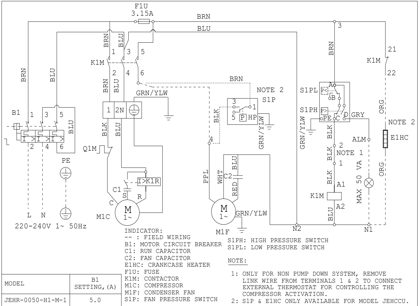
Figure 12: Wiring Diagram JEHR-0050-H1-M-1
