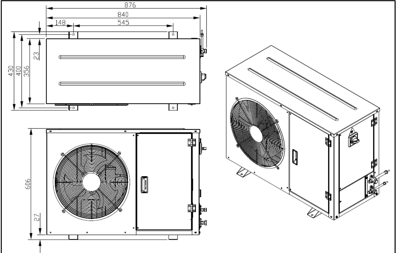
Figure 10: Outline Drawing H1
