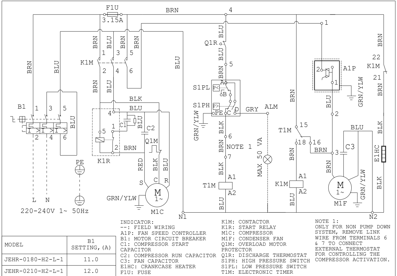
Figure 16: Wiring Diagram JEHR-0180/0210-H2-L-1
