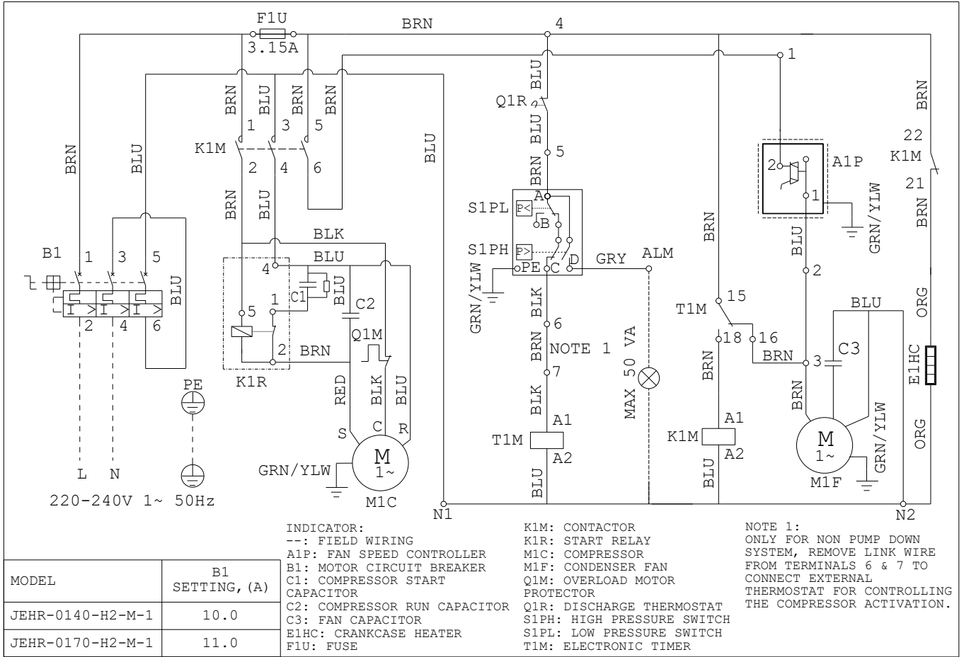
Figure 14: Wiring Diagram JEHR-0140/0170-H2-M-1
