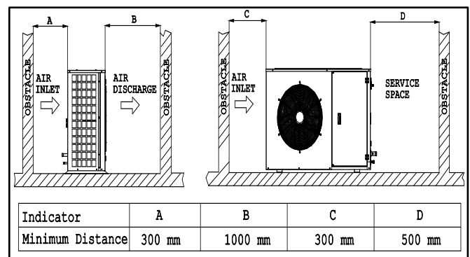
Figure 3: Installation Clearance
