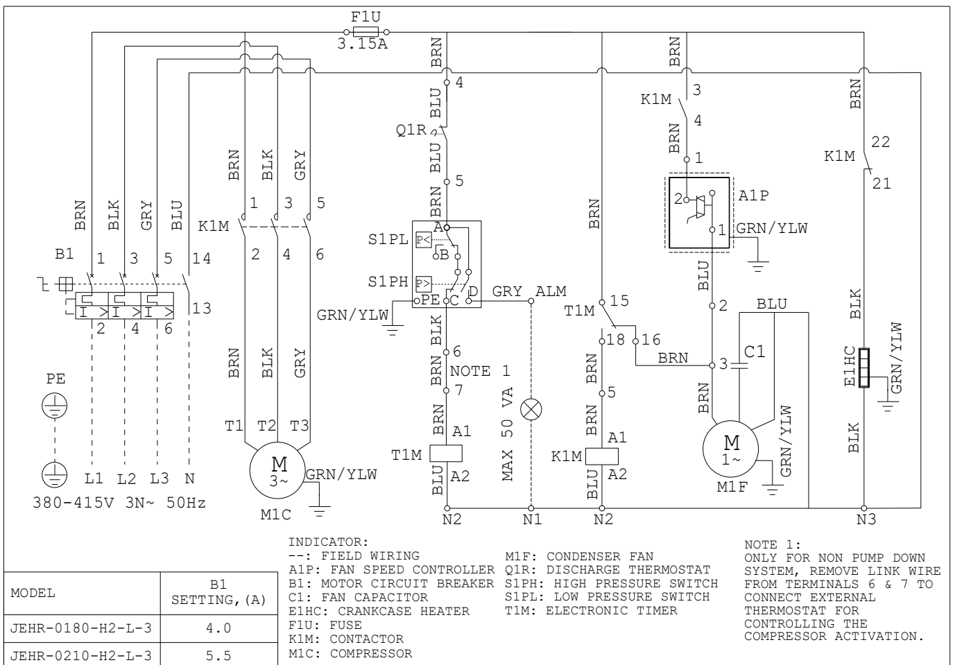
Figure 17: JEHR-0180/0210-H2-L-3
