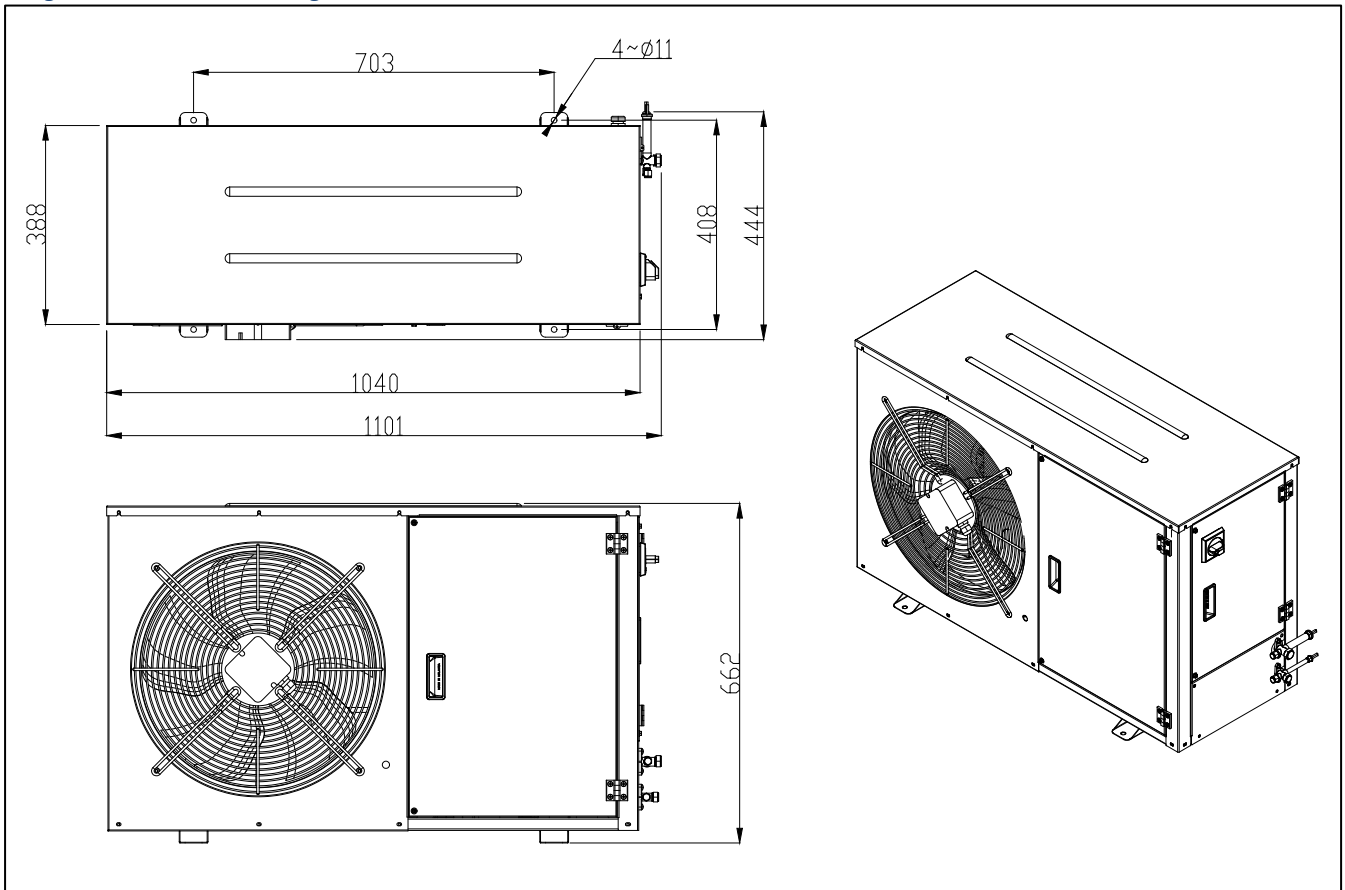
Figure 11: Outline Drawing H2
