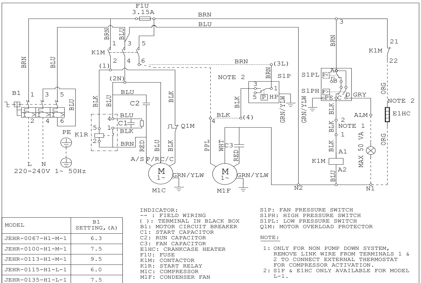
Figure 13: Wiring Diagram JEHR-0067/0100/0113-H1-M-1 & JEHR-115/0135-H1-L-1
