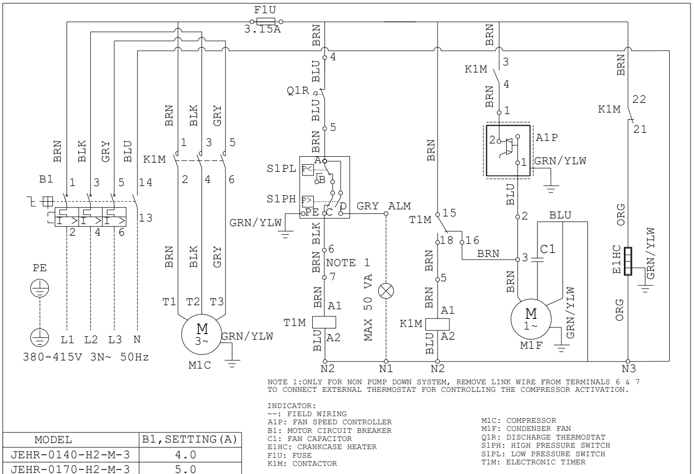
Figure 15: Wiring Diagram JEHR-0140/0170-H2-M-3
