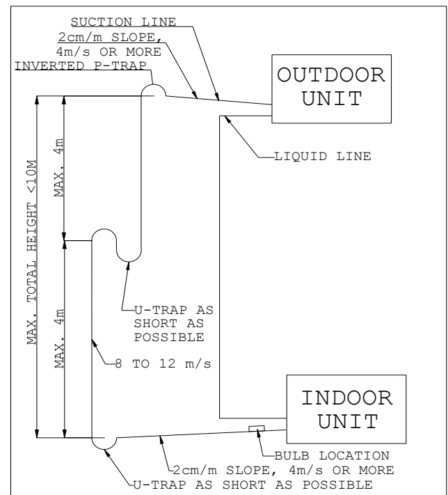
Figure 4: Piping Layout for Outdoor Above Indoor
