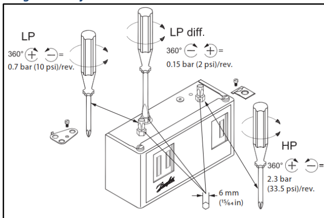
Figure 8: KP17WB: High Pressure Reset Option
