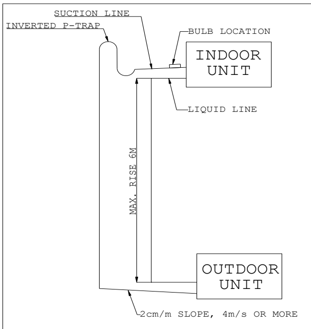
Figure 5: Piping Layout for Outdoor Below Indoor
